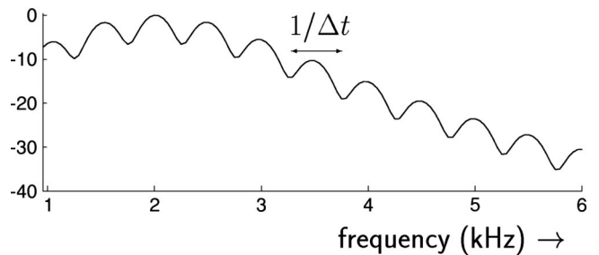
FIG. 14. Part of the observed normalized power spectrum for on-axis observation. Source is located at r=0 m, z=0.25 m, and the observation point is at r=0 m, z=1.25 m. Wave speeds are c_1=250 m/s, c_2=800 m/s. Resulting time delay between the arrivals of the direct wave and the reflected wave is \Delta t=2 ms. As mentioned in Sec. VI, the spacing between the minima should be 1/\Delta t=0.5 kHz, as is indeed the case. Source parameters are \omega_0 = 4\pi \times 10^3 rad s^{-1} , \nu=2 , \alpha=8.71 \times 10^3 s^{-1} , t_r=0.23 ms, and t_w=0.42 ms.
