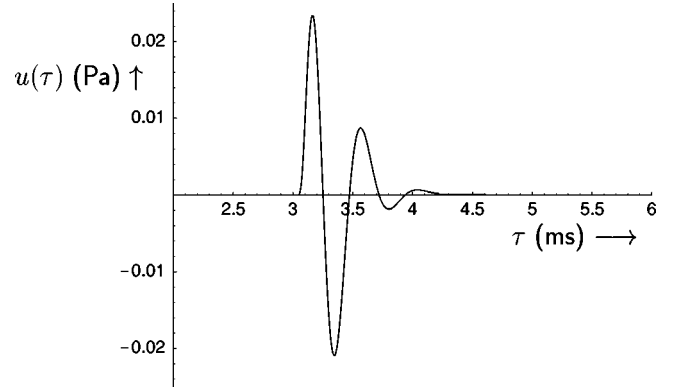
FIG. 8. Total field u(\tau) for the case c_1=500 m/s, c_2=330 m/s. The source is at r=0 m, z=0.3 m. Observation point is at r=1.5 m, z=0.05 m. In this case the direct wave arrival time T_0^{\text{dir}}=3.04 ms and the body-wave arrival time T_1(0)=3.08 ms. Source parameters are \omega_0=2\pi \times 10^3 rad s^{-1} , \nu=2 , \alpha=8.71 \times 10^3 s^{-1} , t_r=0.23 ms, and t_w=0.42 ms.
