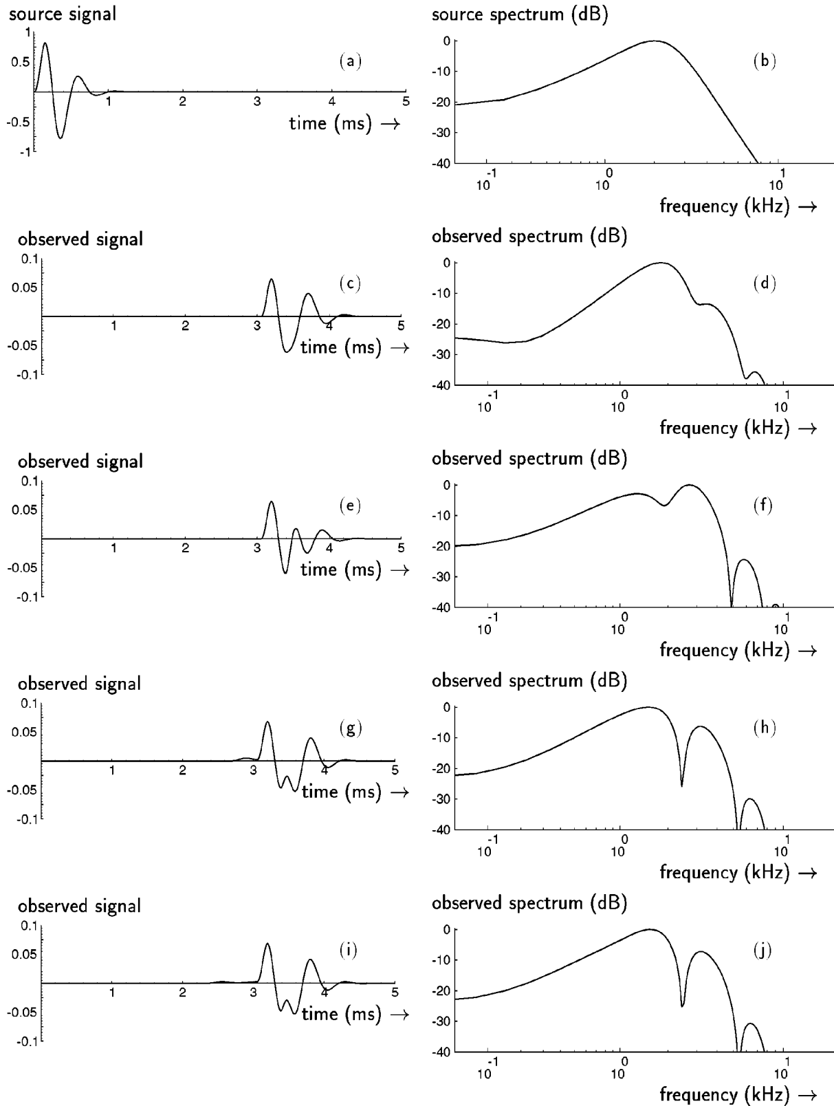
FIG. 15. Source signal (a) and its normalized power spectrum (b). Observed signal and its corresponding power spectrum are shown for different wave speeds in the second medium. In all cases c_1=330 m/s, arrival time of the direct wave is \tau=3.05 ms, and arrival time of the reflected body wave is \tau=3.39 ms. For c_2=200 m/s, there are no head waves (c,d); for c_2=400 m/s, the head waves arrive at \tau=3.36 ms (e,f); for c_2=800 m/s, the head waves arrive at \tau=2.63 ms (g,h); for c_2=1200 m/s, the head waves arrive at \tau=2.29 ms (i,j). Source parameters are \omega_0/2\pi=2\times 10^3 rad s -1 , \nu=2 , \alpha=8.71\times 10^3 s -1 , t_r=0.23 ms, and t_w=0.42 ms. Source is located at r=0 m, z=0.3 m and the observation point is at r=1.0 m, z=0.2 m.
